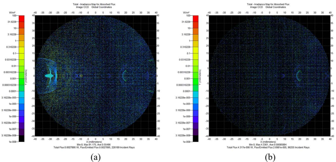
Figure 6. Distribution of stray light on the image plane (a) without a front baffle and (b) with a 60 cm front baffle, both under an irradiance of 1 \text{ W m}^{-2} for the stray light source.
