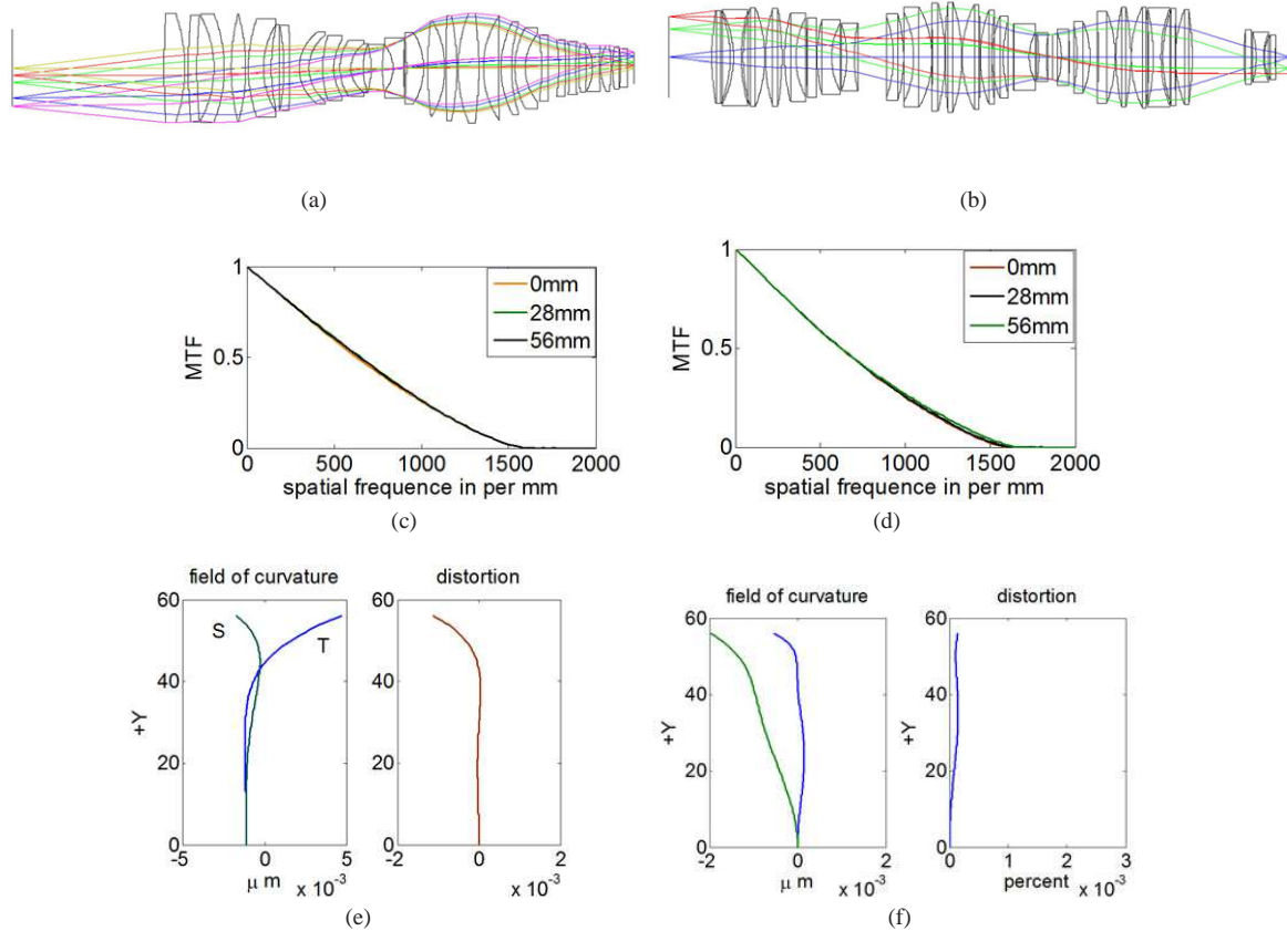
Fig. 8 (a) Design of a lithographic lens system based on the Delano diagram; (b) lithographic lens system of patent #6084723; (c), (e) the MTF, field curvature and distortion of the system in Fig. 8(a); (d), (f) the MTF, field curvature and distortion of the system in Fig. 8(b).
