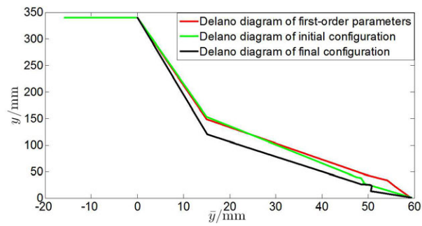
Fig. 5 Plotted values for the first-order parameters, initial configuration, and final configuration derived from the Delano diagram.
