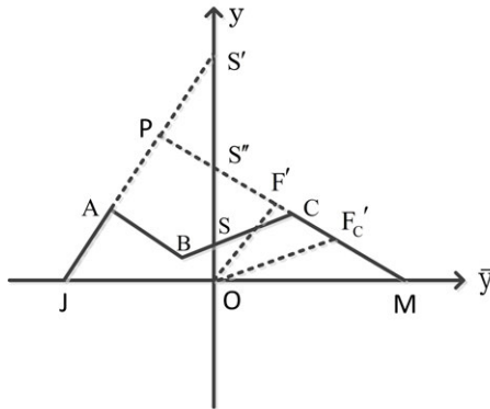
Fig. 1 The Delano diagram of an optical system with three components.
