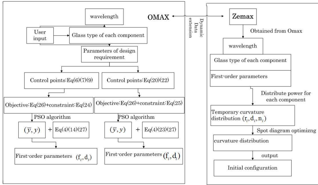
Fig. 4 The process to automatically obtain the initial configuration.
