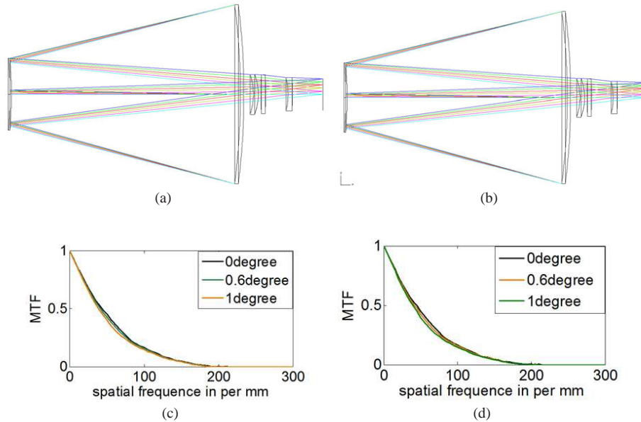
Fig. 6 (a) Initial configuration generated by OMAX; (b) final configuration optimized from Fig. 5; (c) Modulation Transfer Function (MTF) of the initial configuration; (d) MTF of the final configuration.
