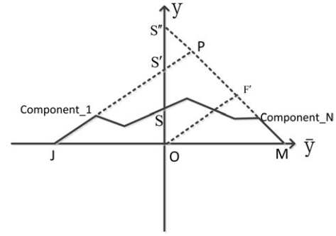
Fig. 2 Control points of a system with a finite object distance are shown in the Delano diagram.
