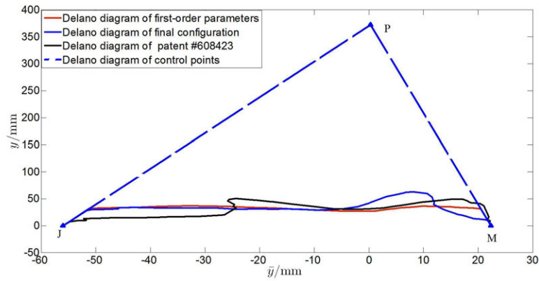
Fig. 7 Delano diagram of the first-order parameters, final configuration, patent configuration, and control points of the lithographic lens system.
